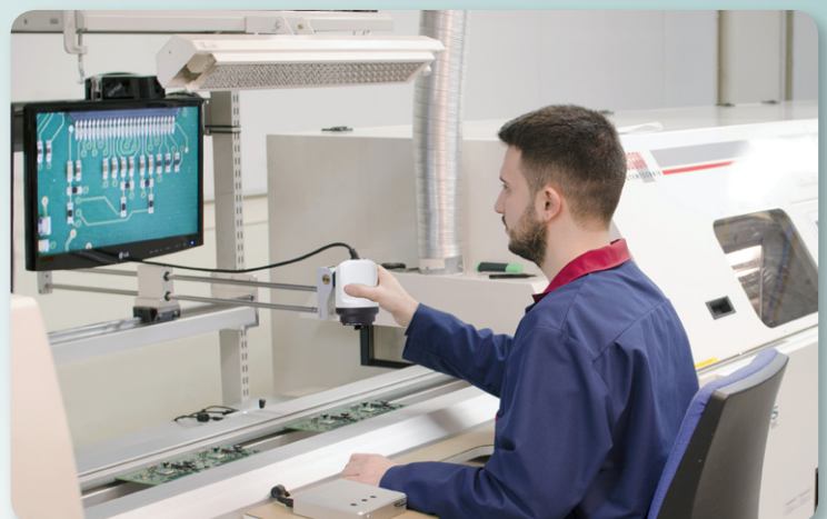
M30x-HD system with 4-directional tilt device and In-Line XY-stand mounted over conveyor in a SMT production line .
