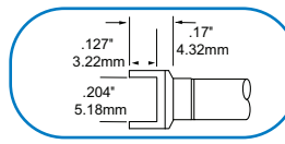
RFP-DL1 Tunnel Cartridge SOIC-14-16 Length 10.16mm (0.4")
