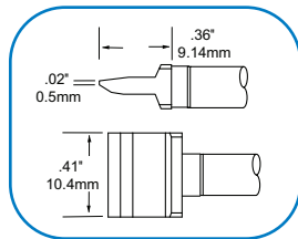
RFP-BL1 Blade Cartridge Length 10.4mm (0.41")
