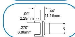
RFP-DL3 Tunnel Cartridge SOMC-16 Length 11.15mm (0.44")
