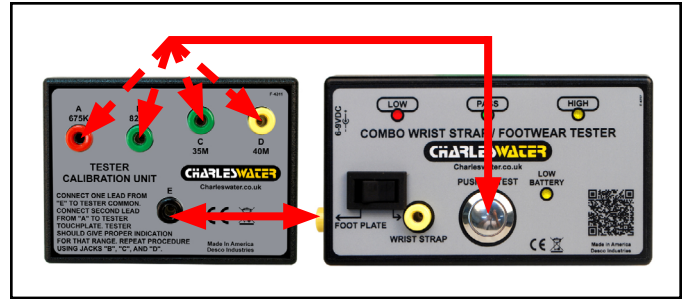
Figure 5. Verifying the calibration of the footwear circuit in the Combo Tester
